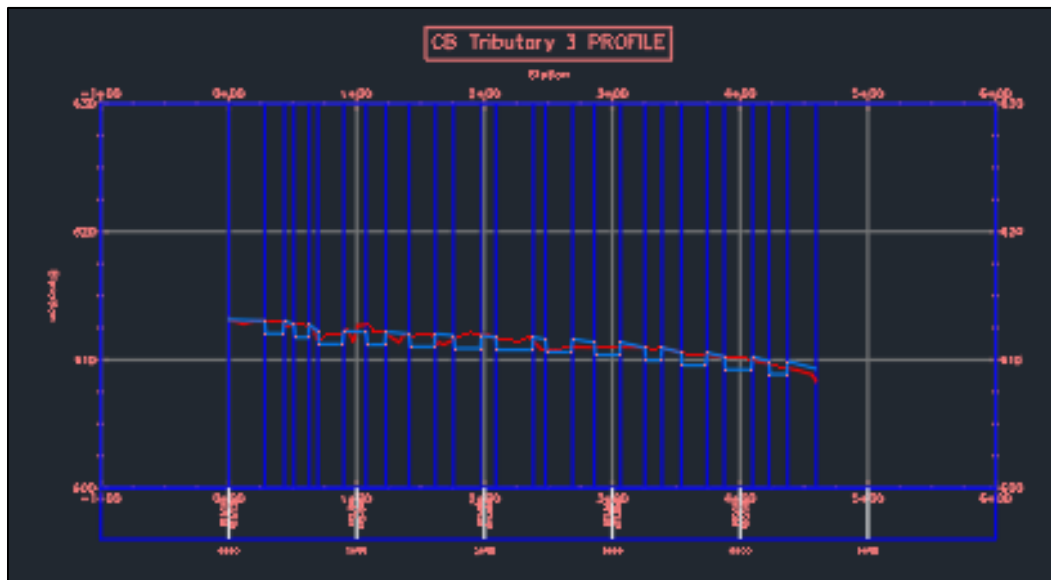
Figure 24: Vertical Profile with Riffle/Pool Sequence, Tributary 3
