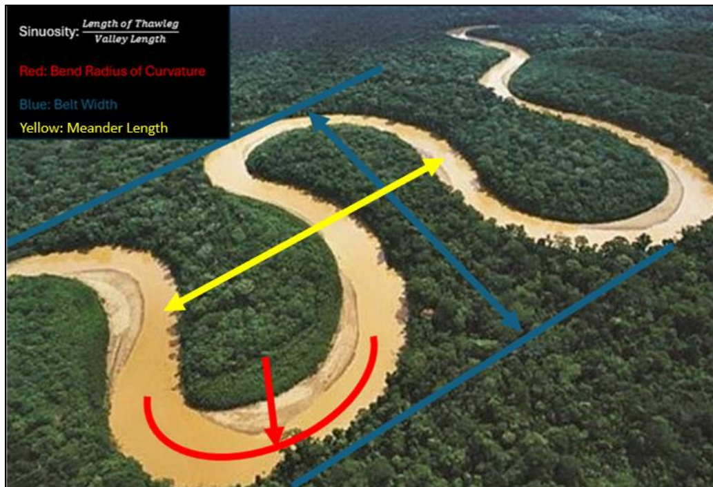
Figure 3: Plan Form Geometry Characteristics
